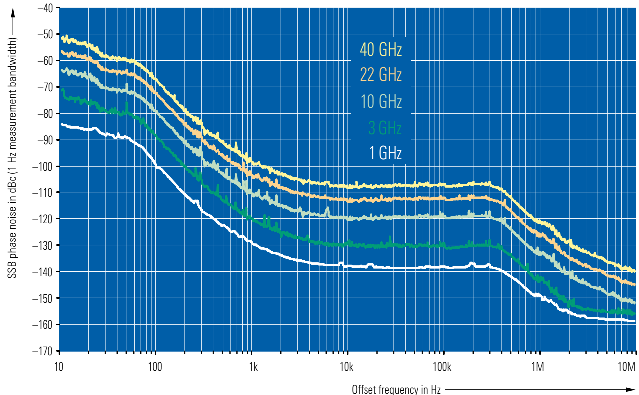
Single sideband phase noise for various frequencies (each with the R&S®SMF-B1 OCXO reference oscillator option)
