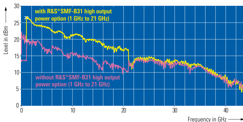
Maximum output power with and without the high output power option in the frequency range 100 kHz to 43.5 GHz (with R&S®SMF-B27 step attenuator). The lower curve in the frequency range 100 kHz to 1 GHz is with activated pulse modulator of the R&S®SMF-B2 frequency extension
